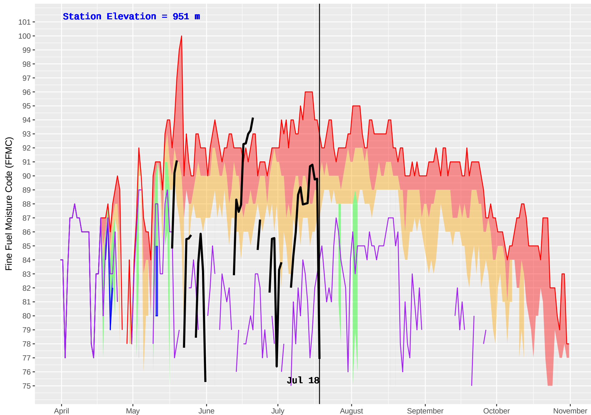
NORTH BABINE (173) : Historical (1986–2016) and Current (2018) Daily Fine Fuel Moisture Code (FFMC)
