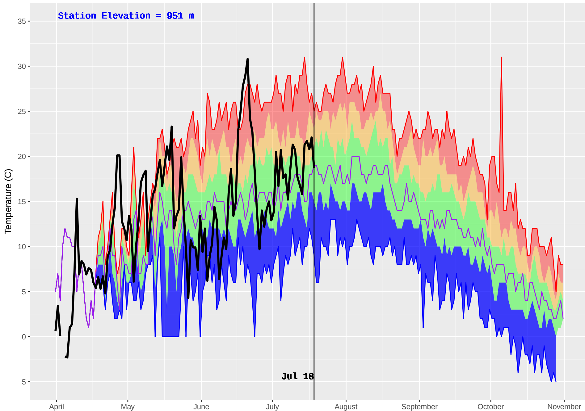
NORTH BABINE (173) : Historical (1986–2016) and Current (2018) Daily Temperature
